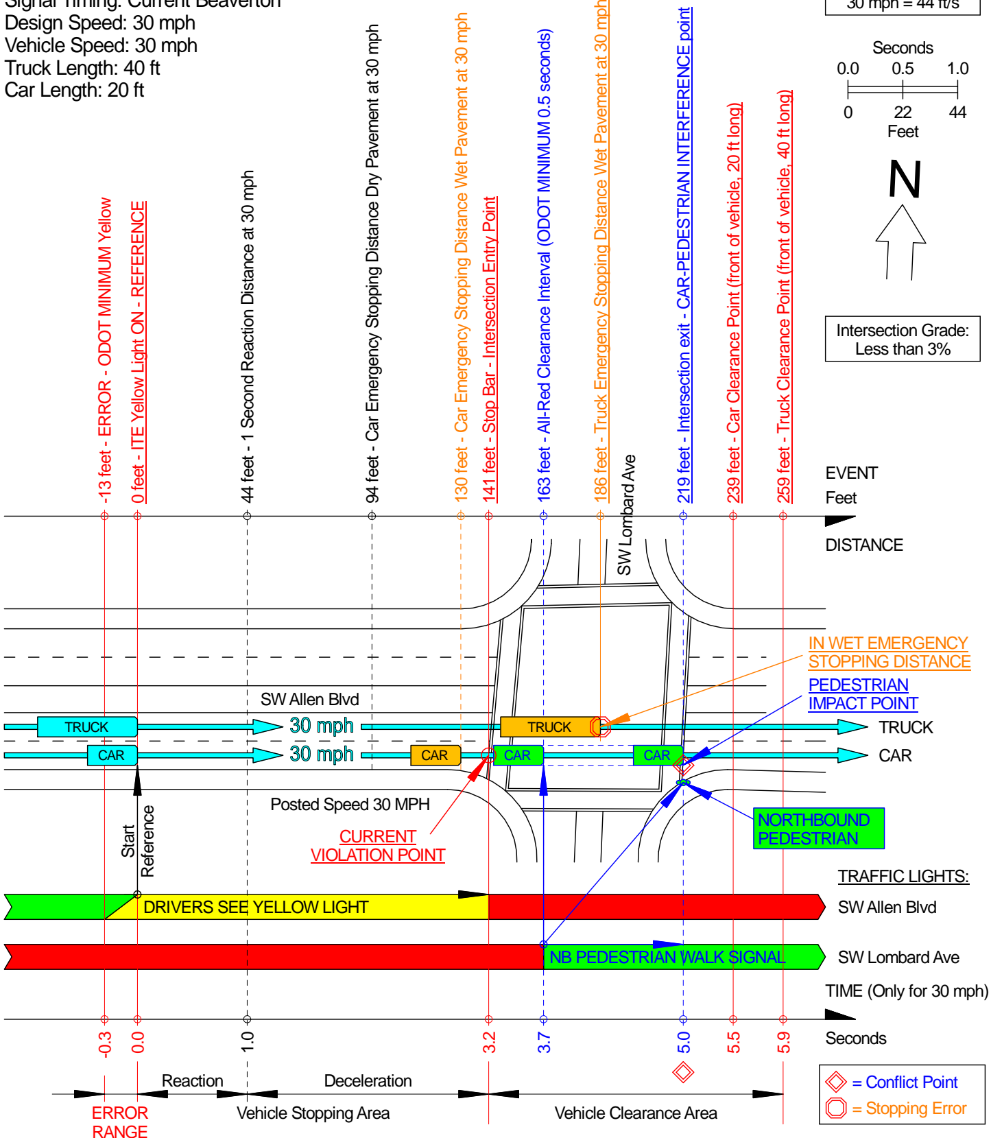
30 MPH VEHICLE Speed Current Beaverton Yellow Change Interval EB SW Allen Blvd, Beaverton Scaled drawing showing vehicle stopping distances, interference(s), violation point(s) and errors related to intersection and traffic signals. (Rev. 17, April 15, 2014)
