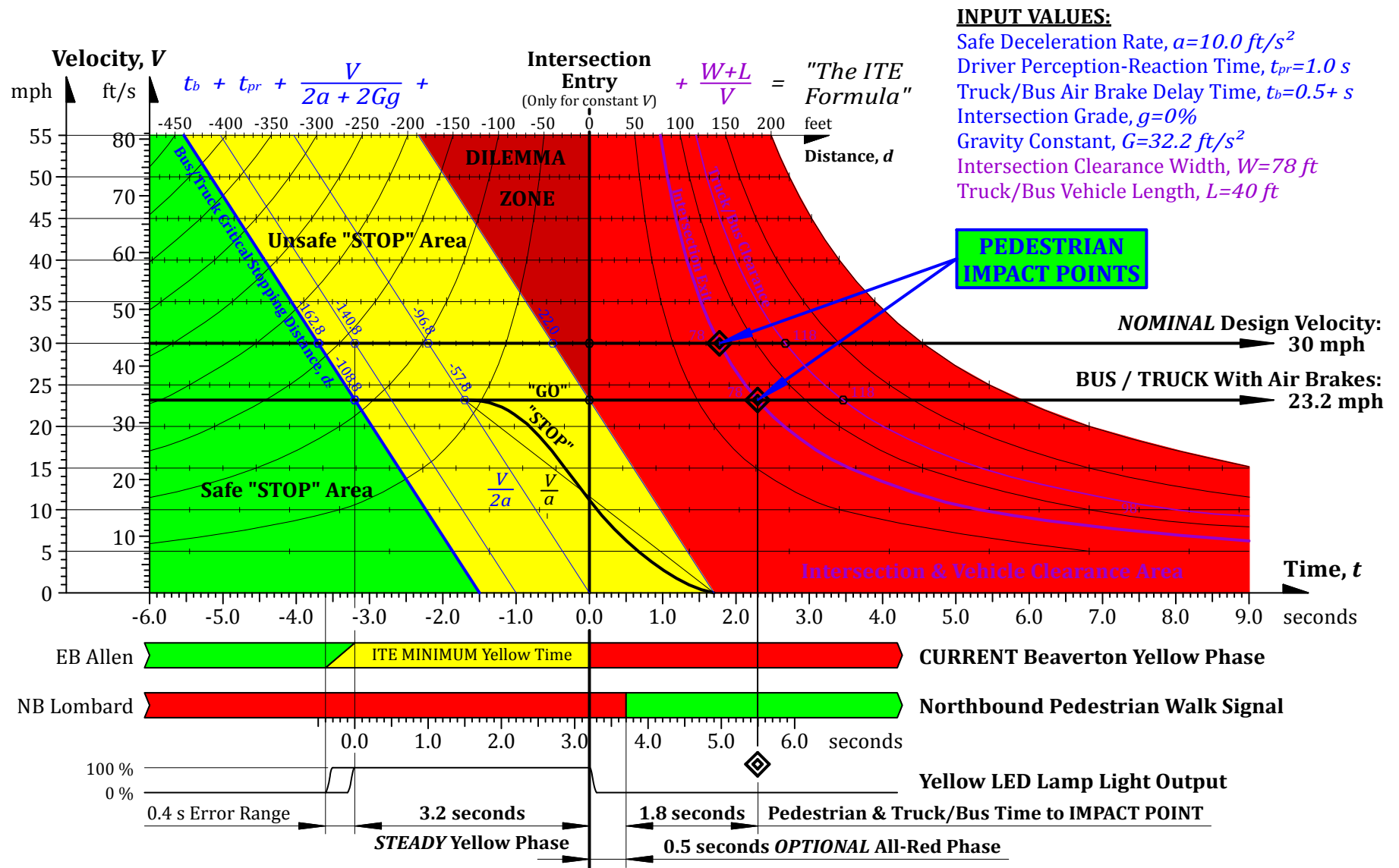
Shown Examples: CURRENT Yellow Timing for 23.2 and 30 MPH Eastbound SW Allen Blvd. at SW Lombard Ave. Beaverton, Oregon Air Brake Dilemma Zone - Velocity vs. Time & Distance Yellow Traffic Light Vehicle Motion Graph
